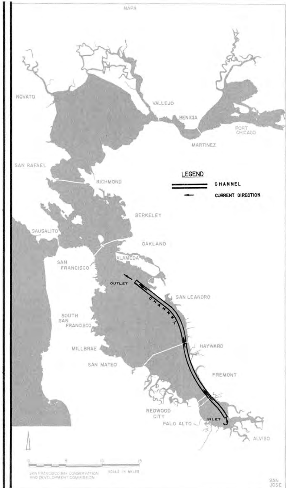
FIGURE 1 Longitudinal Barrier and Channel along East Shore
