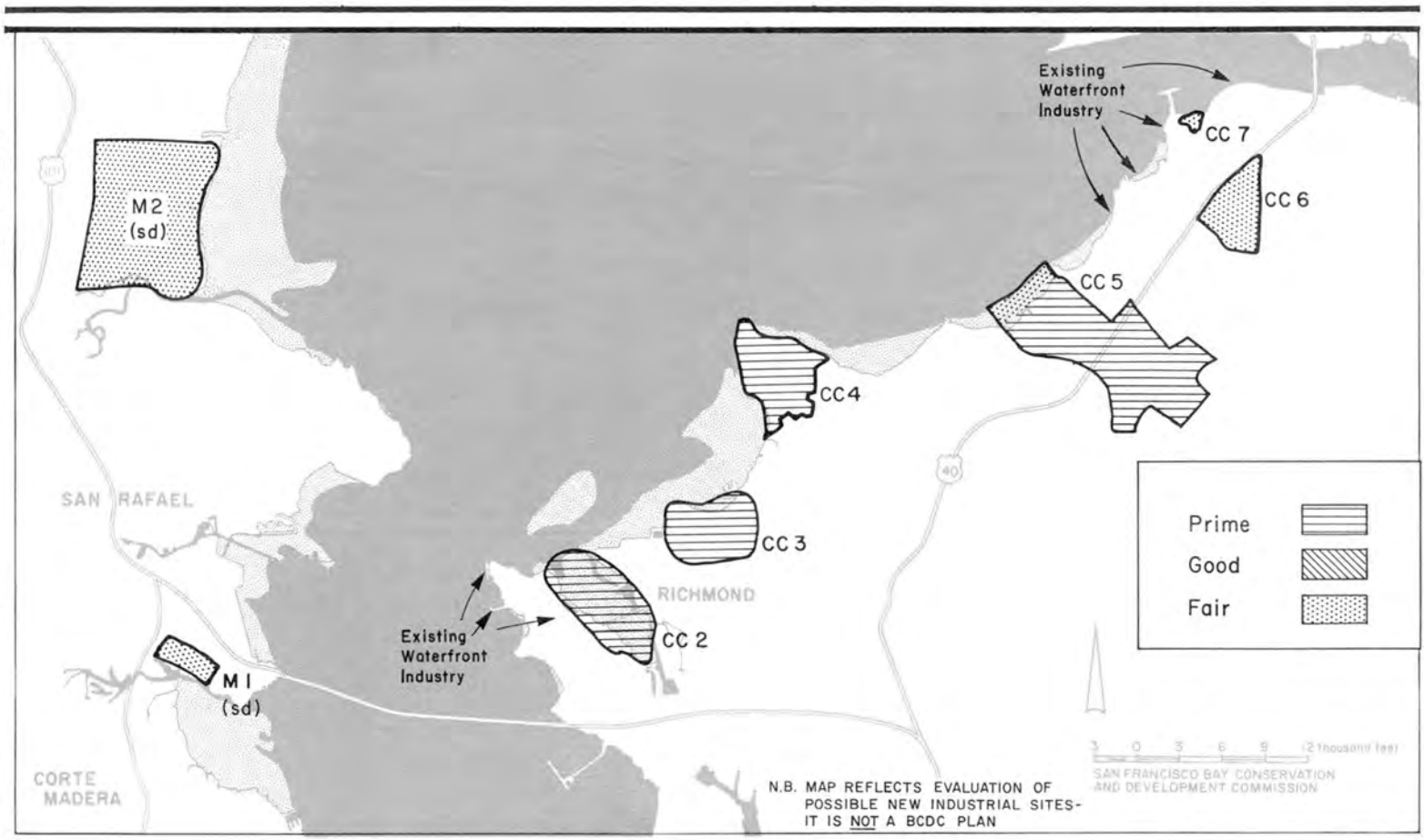
FIGURE 3 Possible New Sites for Waterfront Industry: San Pablo Bay (south portion)
