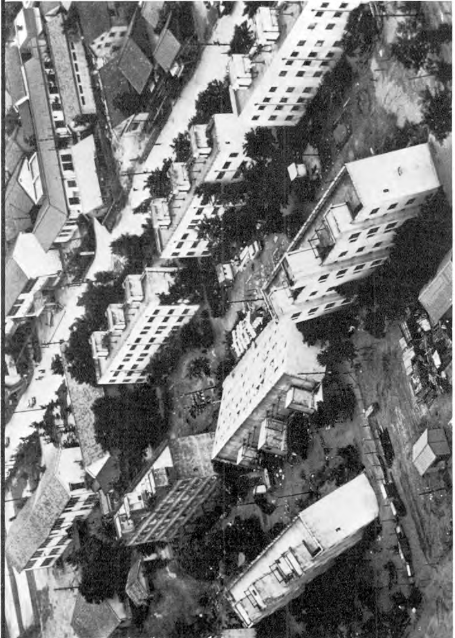
FIGURE 1 Tilting of Apartment Buildings at Kawagishi-cho, Niigata
