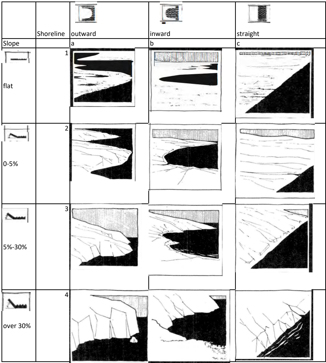
FIGURE 1 Basic Land-Water Classifications
