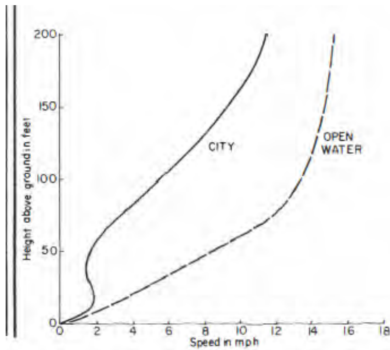
FIGURE 1 Typical Wind Speed Distributions in the Vertical
