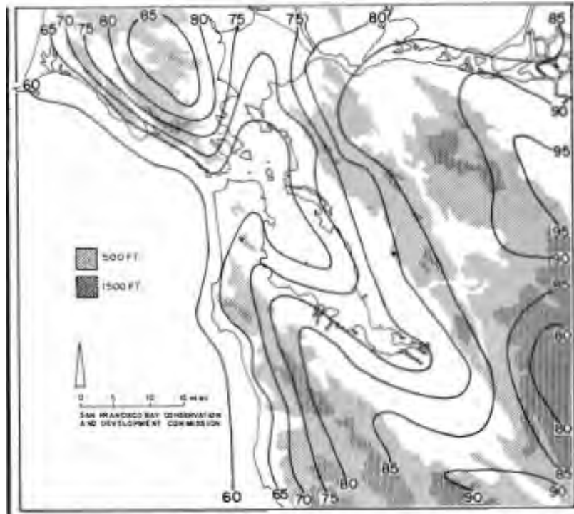
FIGURE 3 Daily Mean Maximum Temperature for July 1951-1960 (° F)
